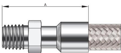
NPT陽螺紋
