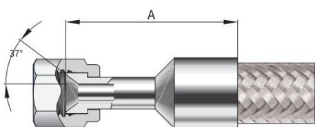
SAE 37°(JIC)內旋
